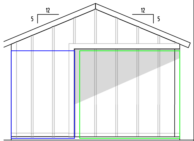
Left Elevation
